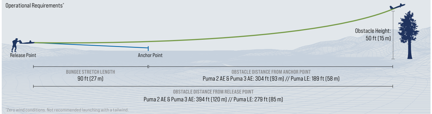
Bungee Adapter for Puma 2 AE and Puma 3 AE
